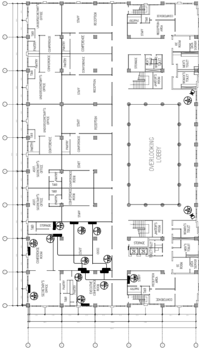
BUILDING 2 SECOND FLOOR PLAN SCALE 1/4" = 1'-0"
